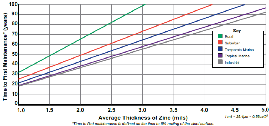
Figure 3: Time to First Maintenance for Hot Dip Galvanized Bridges 3
