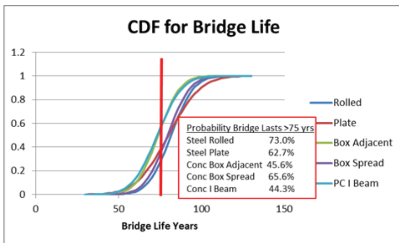
Figure 1: Cumulative Density Function of Bridge Life
